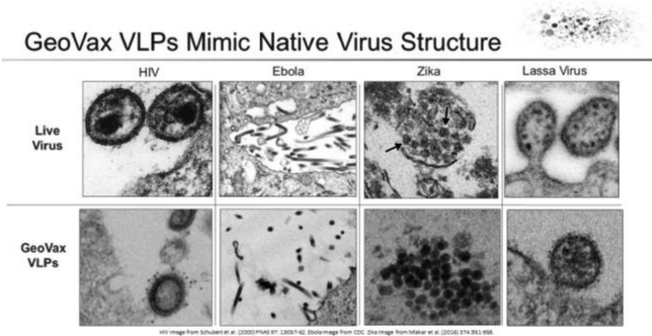
Figure 1. Comparison of MVA-VLPs and native virus structures
